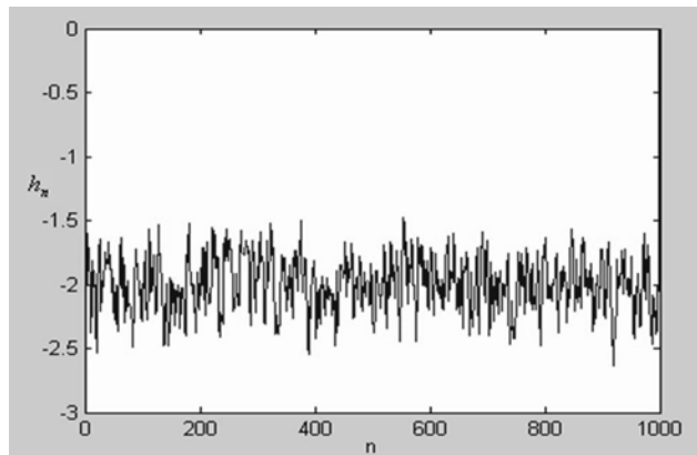
Fig. 3. Simulation of ARMA(1,1) model of h_n = a_0 + a_1 h_{n-1} + b_1 \varepsilon_{n-1} + \sigma \varepsilon_n , where a_0 = -1 , a_1 = 0.5 , b_1 = 0.1 , and \sigma = 0.1
