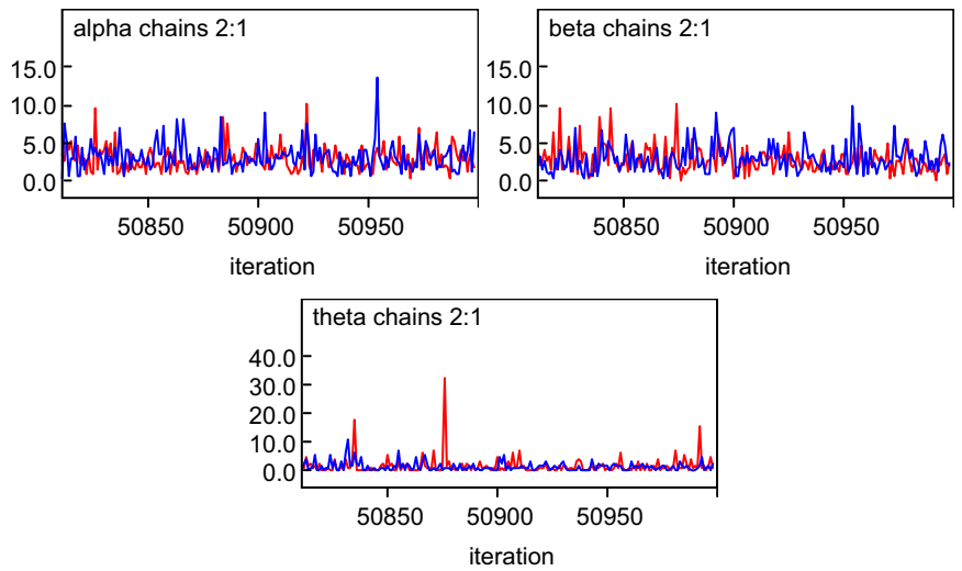
Fig. 2. Convergence tools for monitoring stationarity of MCMC
