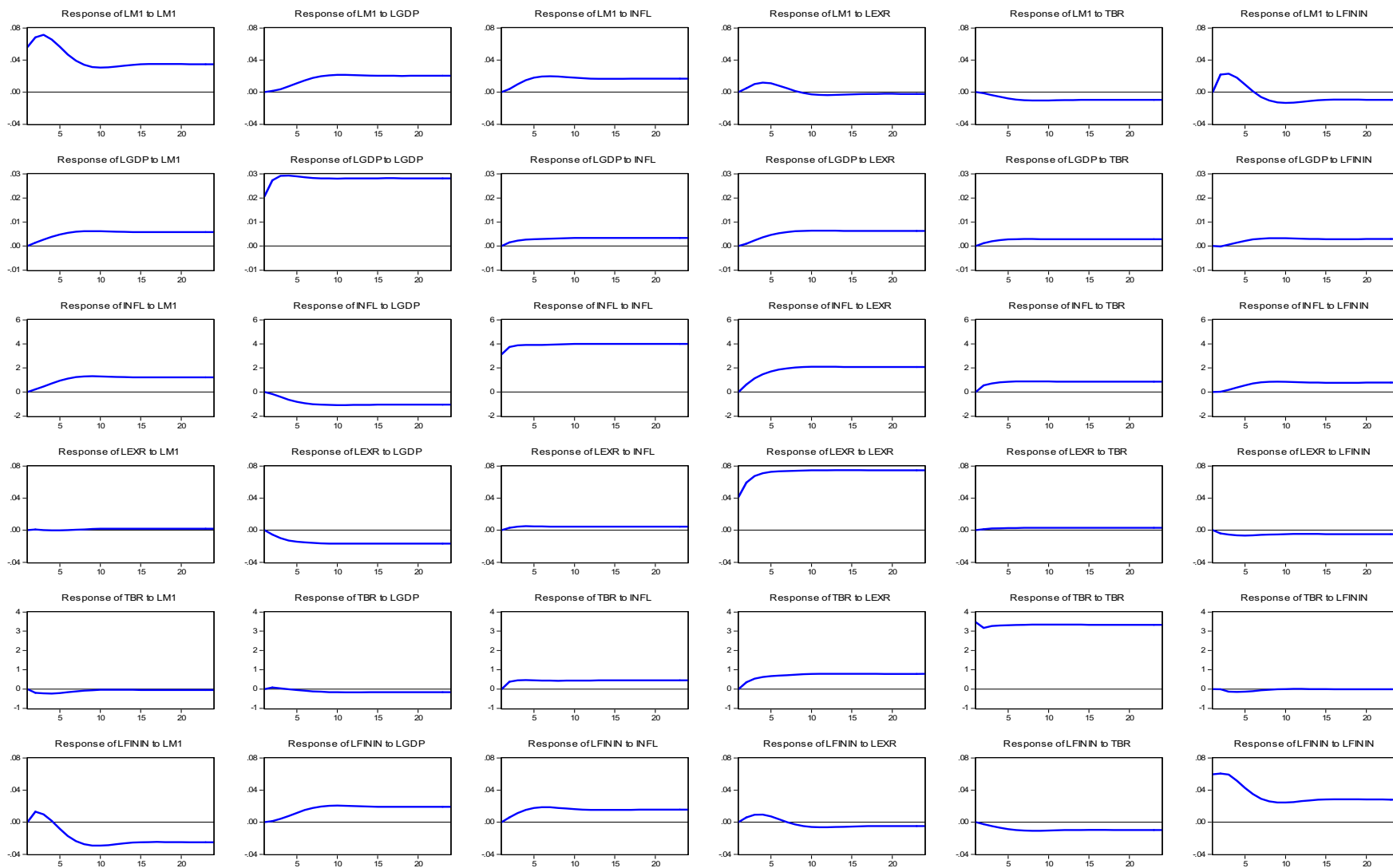
Fig. 2. Impulse response functions
