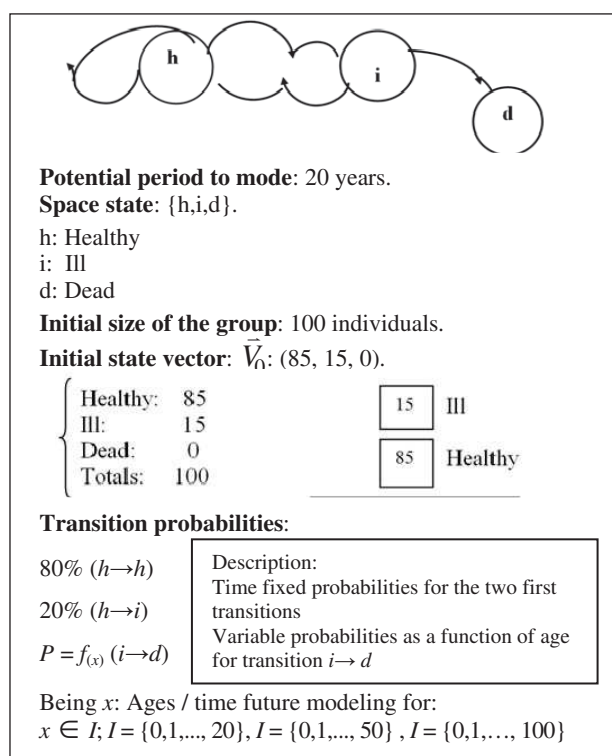
Fig. 1. Markovian graph
