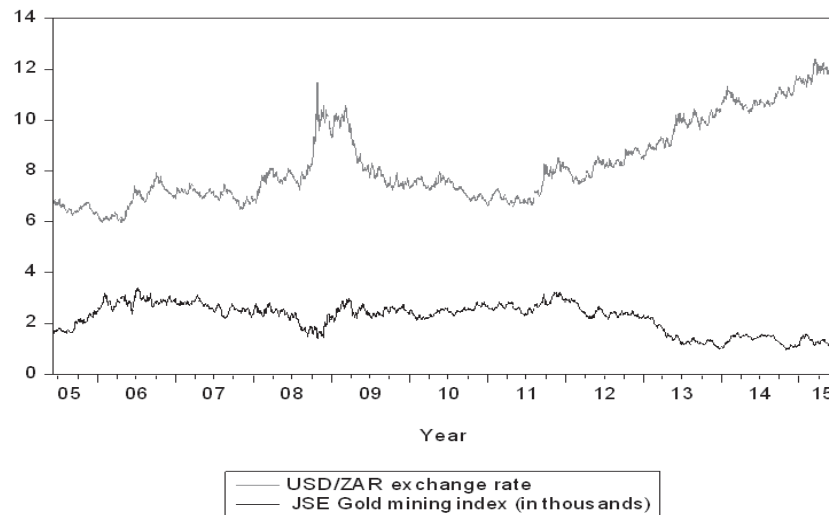
Fig. 1. Time series plot of daily gold mining index and USD/ZAR exchange rate
