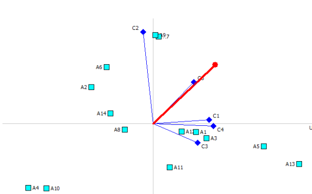
Figure 3. PROMETHEE GAIA
