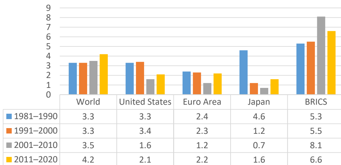
Figure 1. Average GDP (actual and predictions)
