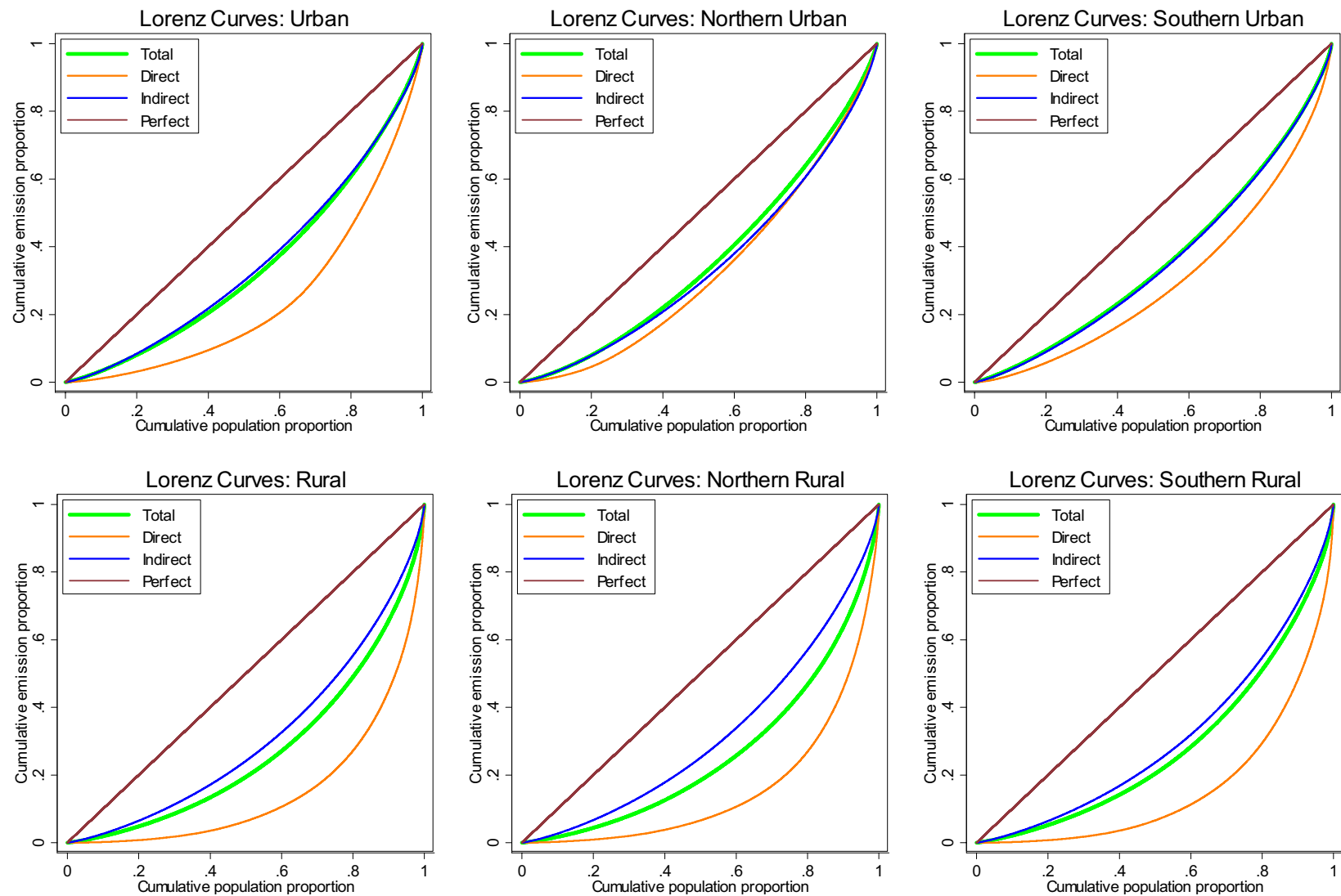
Fig. 12. Lorenz curves of urban and rural per capita CO 2 emissions (all, north, south)
