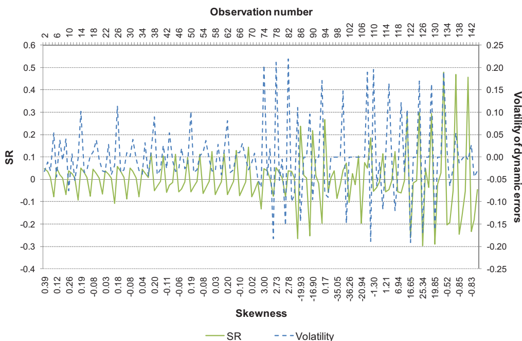
Fig. 6. Changes in Sharpe ratios and dynamic errors' volatility
