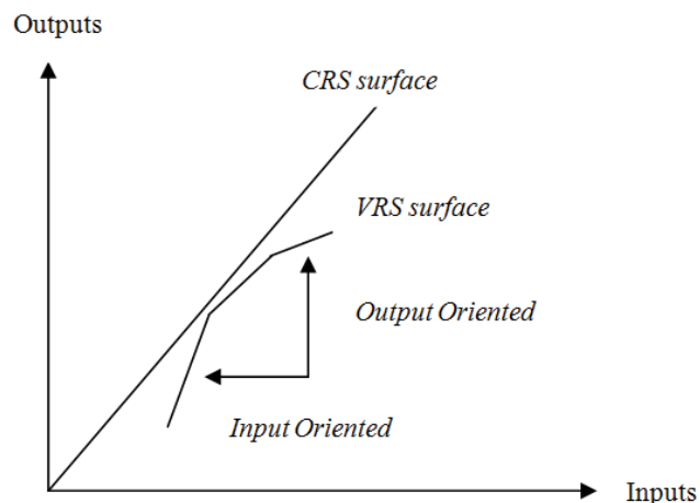
Fig. 1. Envelopment surface in DEA analysis and its orientation for the DMUs
