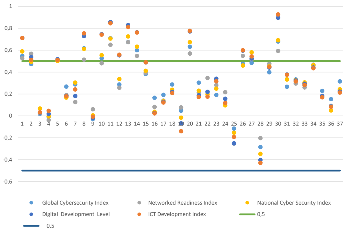
Figure 2. Results of correlation analysis
