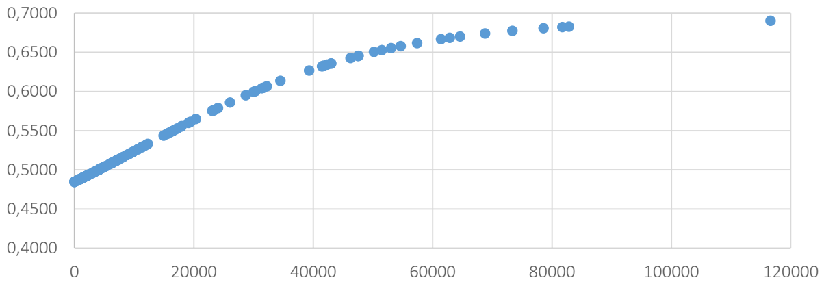
Figure 3. Graph of the second type of the curve for GDP per capita
