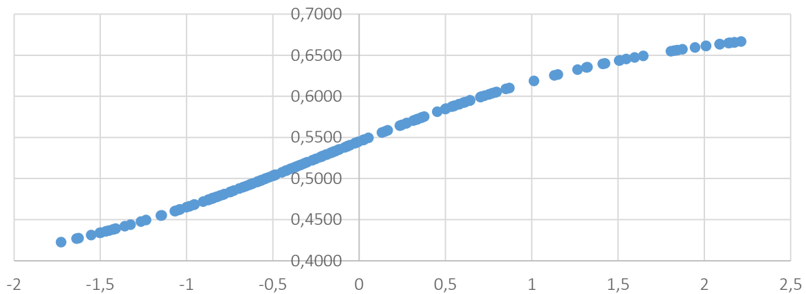
Figure 4. Graph of the first type of curve for Control of corruption: estimate
