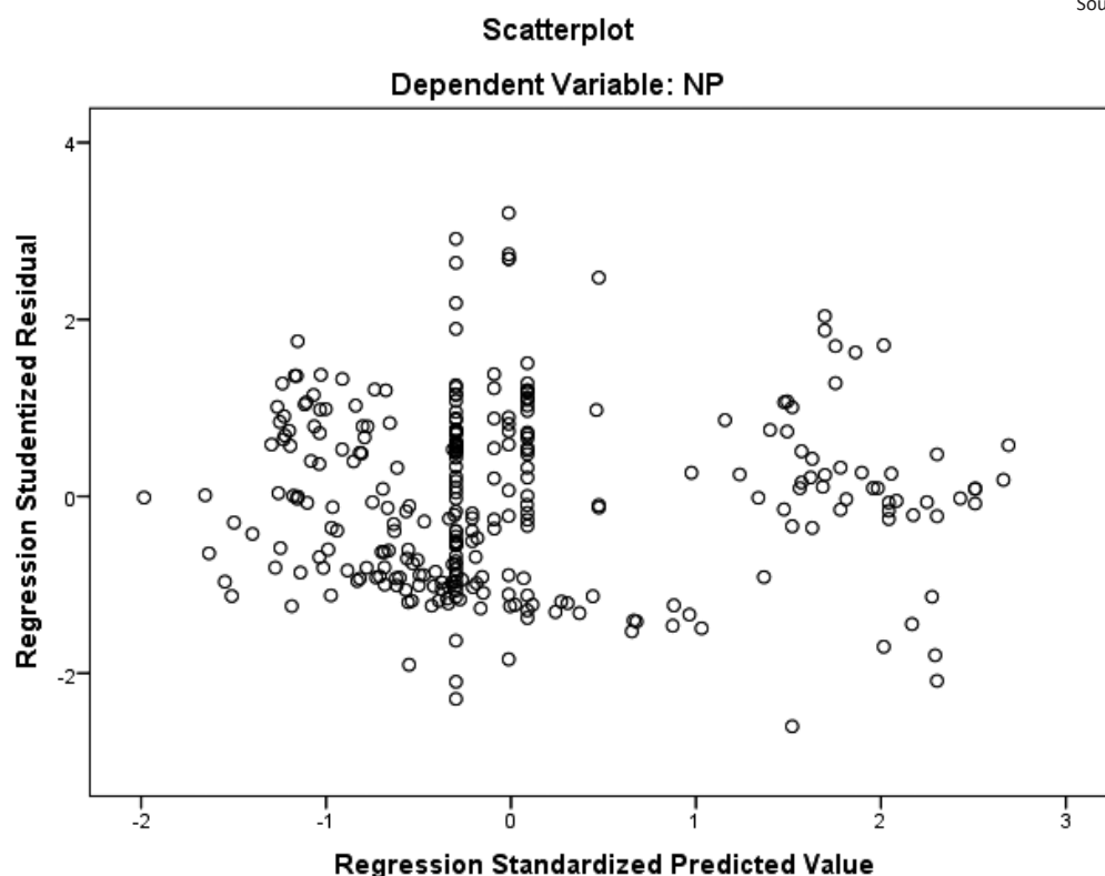
Figure 5. Heteroscedasticity test
