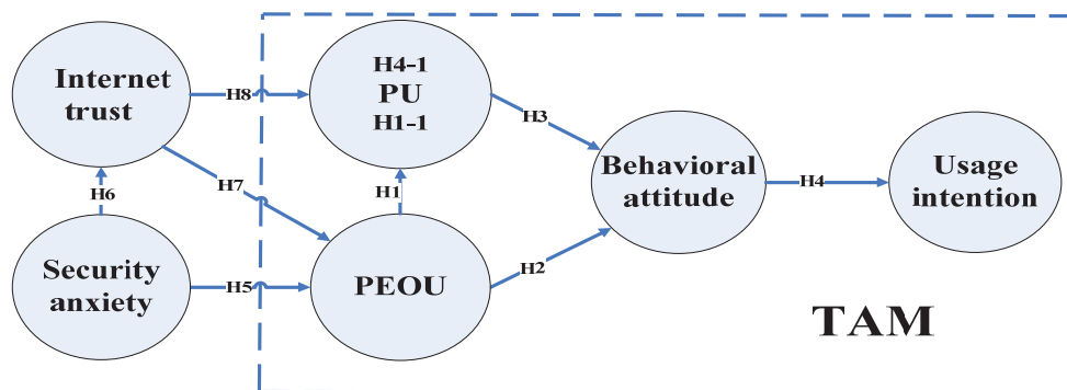
Fig. 1. Research model
