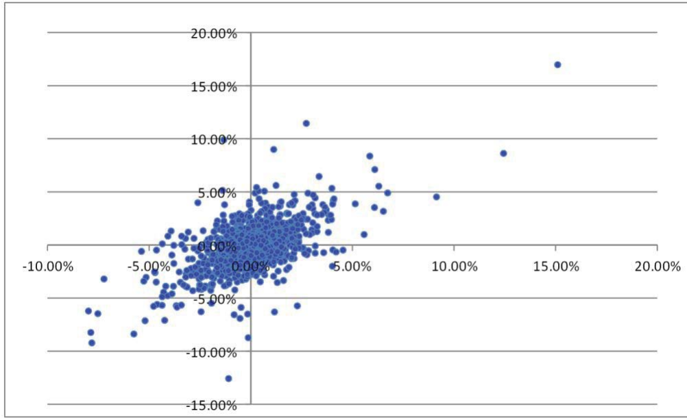
Fig. 1. Scatter plot of AT&amp;T vs. MSFT returns
