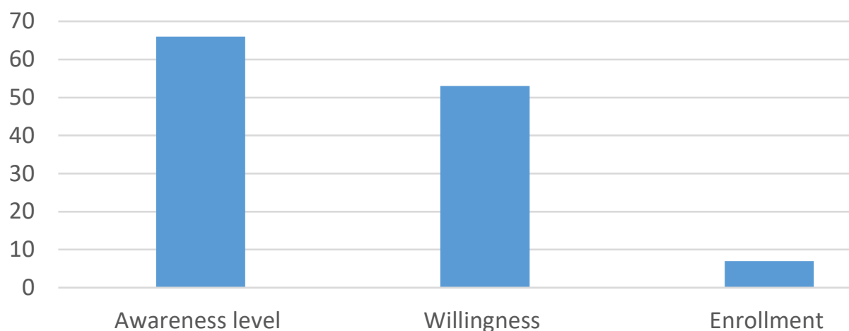
Figure 1. Descriptive statistics
