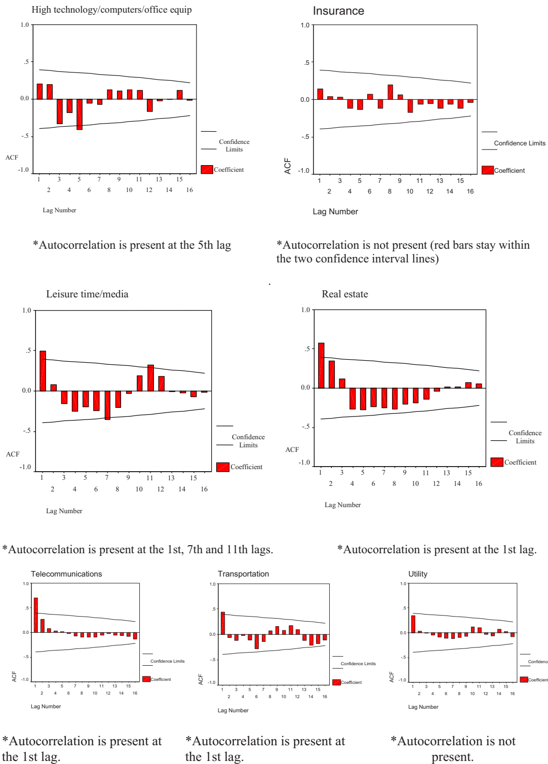
Fig. 2. Intra-Industry Default Correlations (SPSS automatically uses 16 lagged values as the default)
