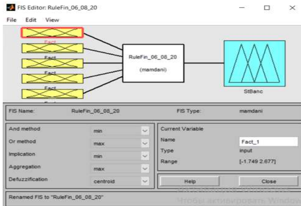
Figure 2. The Mamdani model constructed
