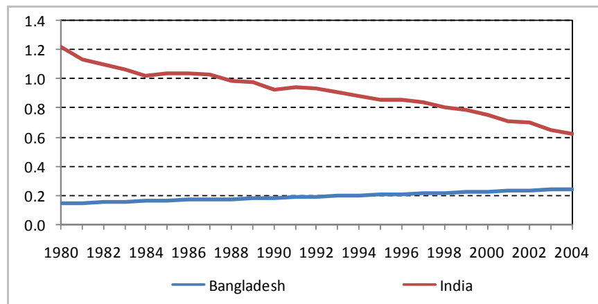
Fig. 3. CO 2 emissions (kg per PPP $ of GDP)
