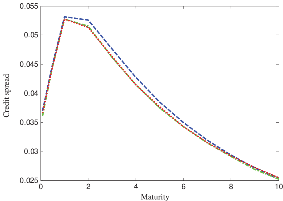
Note: (–) denotes Model 1; (– –) denotes \rho = 0.9 ; (··) denotes \rho = 0.6 .
