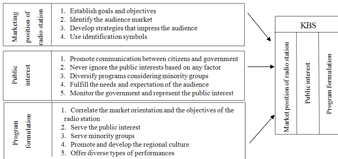
Fig. 1. Research framework
