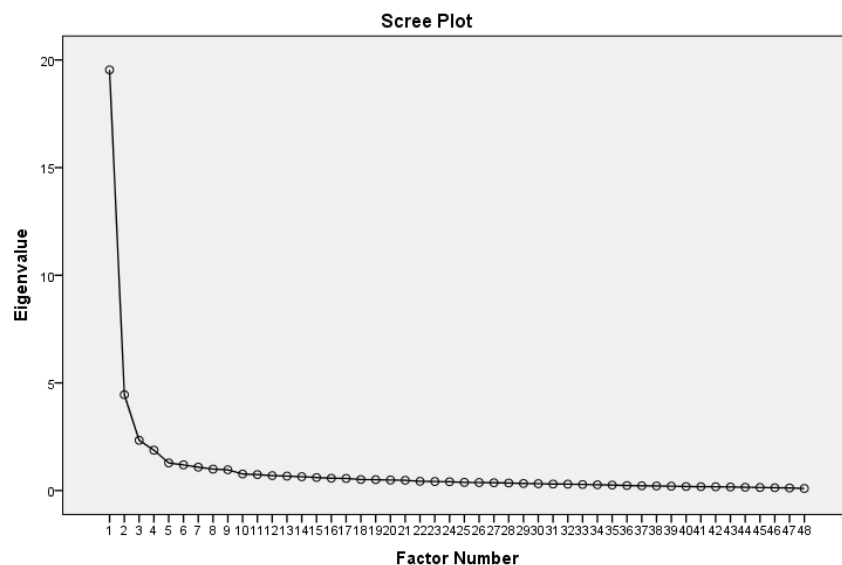
Fig. 2. Scree plot
