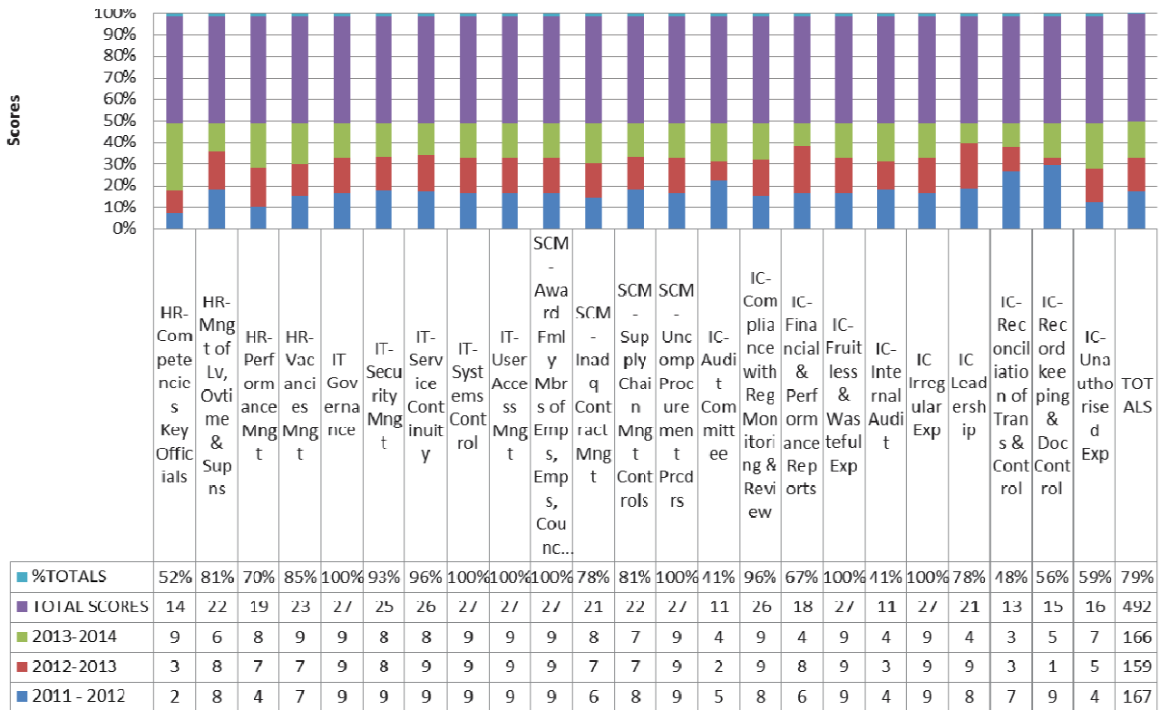
Fig. 6. Overall scores
