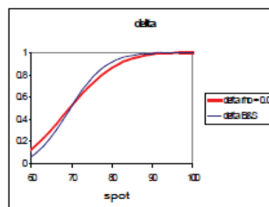
Fig. 12. The B&amp;S delta hedging strategy
