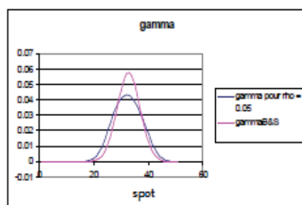
Fig. 11. The B&amp;S gamma hedging strategy
